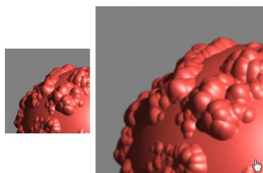
Mitchell-Netravali
