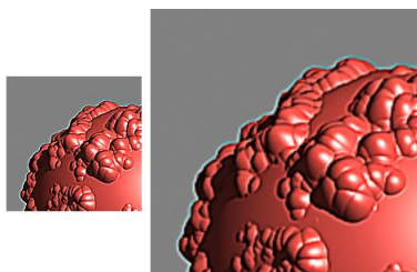
Mitchell-Netravali, ringing=2.0
