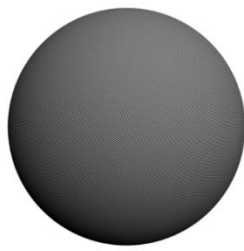
Quadratic filter
