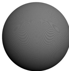
Catmull-Rom
