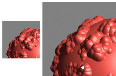
Catmull-Rom
