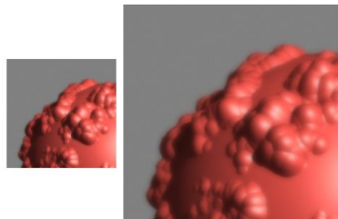
Blend filter
