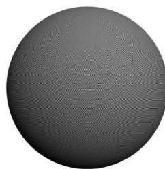
Blackman
