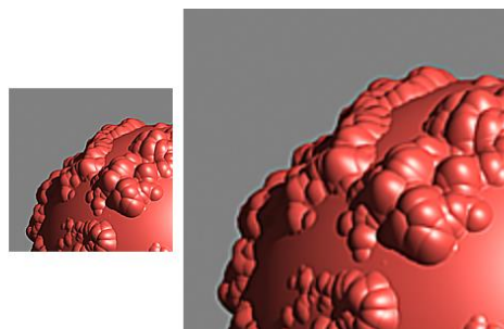
Mitchell-Netravali, ringing=1.5
