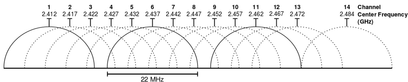
Figure 1. The 2.4GHz spectrum is so crowded and has so few usable channels (image from Wikipedia).
