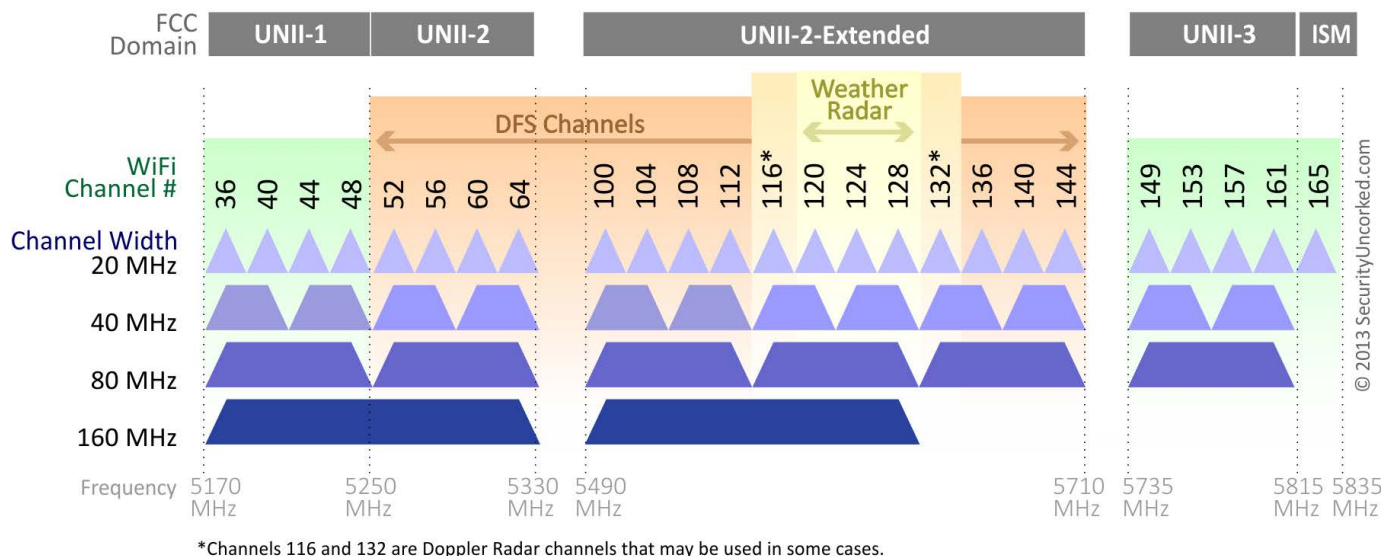
Figure 2. The 5GHz Channel Allocation (image from http://securityuncorked.com )
